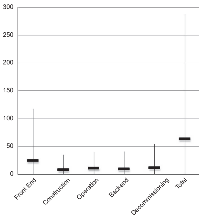
Fig. 3. Range and mean emissions reported from qualified studies for the nuclear fuel cycle ( \text{g CO}_2\text{e/kWh} )
